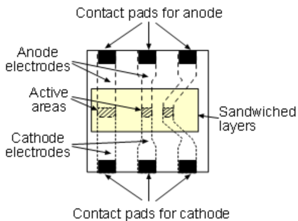
Possible device designs
