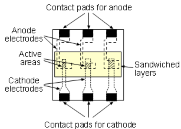
Presently used device designs
