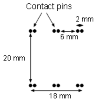
Design of contact pins at the platform of solar simulator
