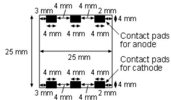
Design for contact pads on the substrate
